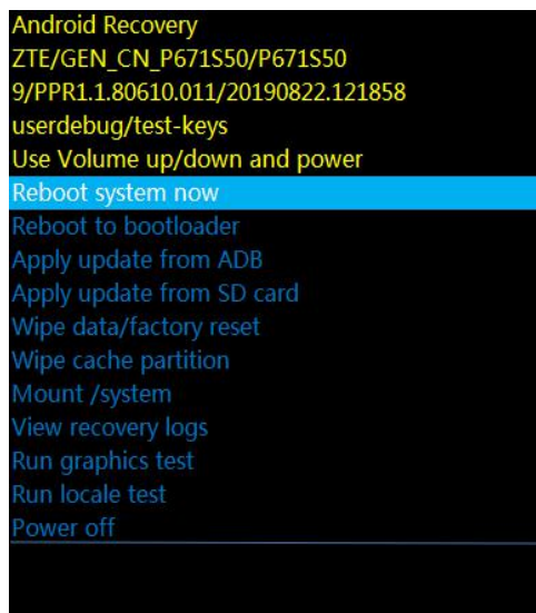
图 3-2 Recovery 菜单
